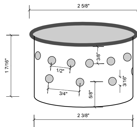
Fig 2: Super Cat stove dimensions
